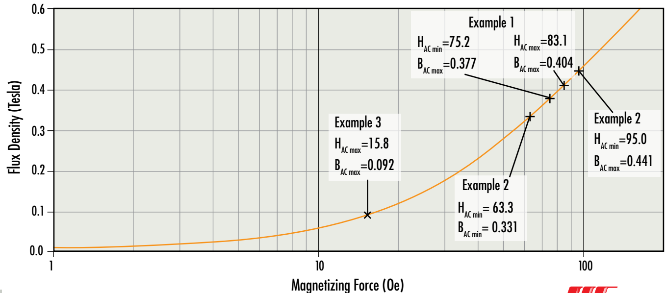
60 \mu Kool M \mu DC Magnetization Curve
