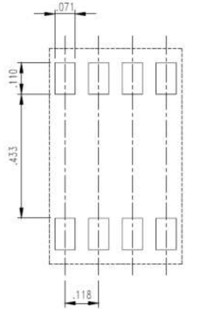
PROPOSED PAD ARRANGEMENT
